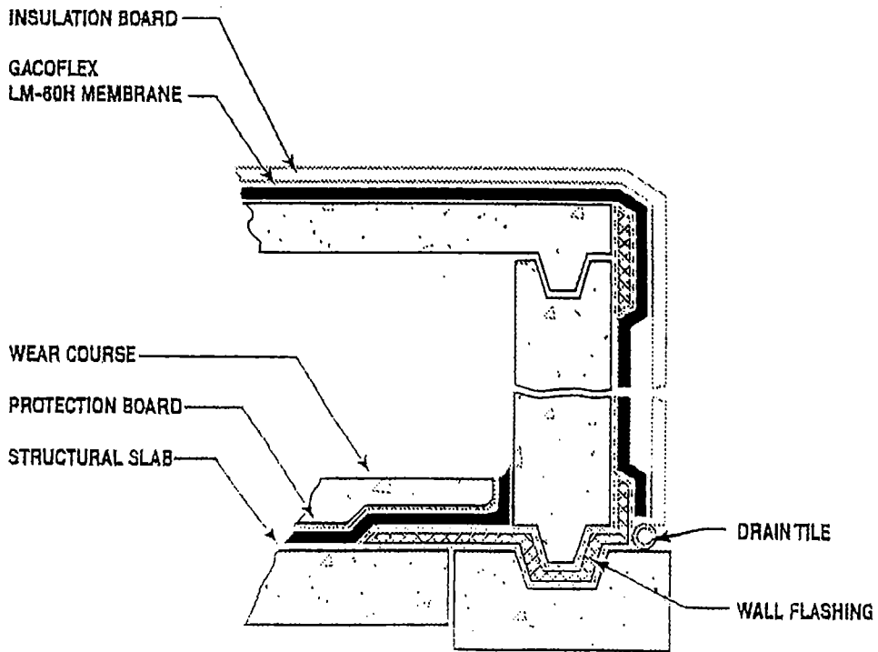
DETAIL FOR CONCRETE UNDERGROUND STRUCTURES
