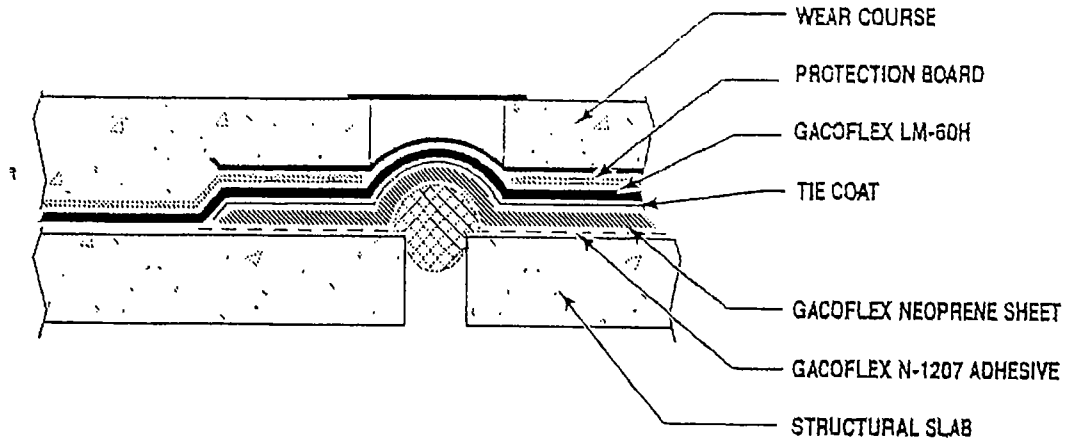
EXPANSION JOINT
